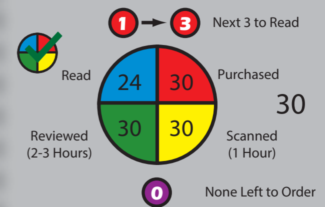
Six Sigma Statistical Analysis Using Excel and Minitab
